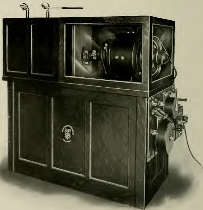
Fig. 15. Interrupterless coil.
